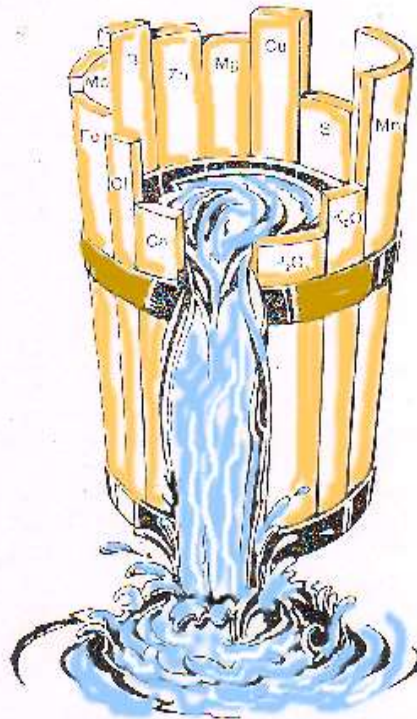
Liebig's "Law of the Minimum"
